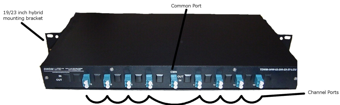
Figure 1: An 8 channel Dual Fiber DWDM showing the common parts of all Telecom Engineering DWDM/CWDM/WDM Lite™ Products
