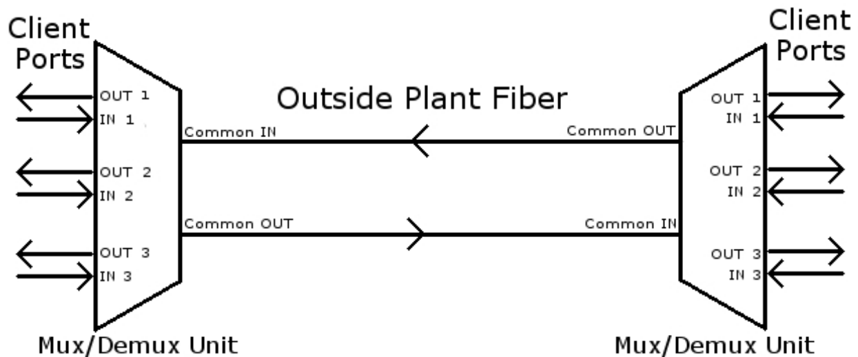
Figure 2: A diagram of a dual unit DWDM/CWDM/WDM system over two fibers
